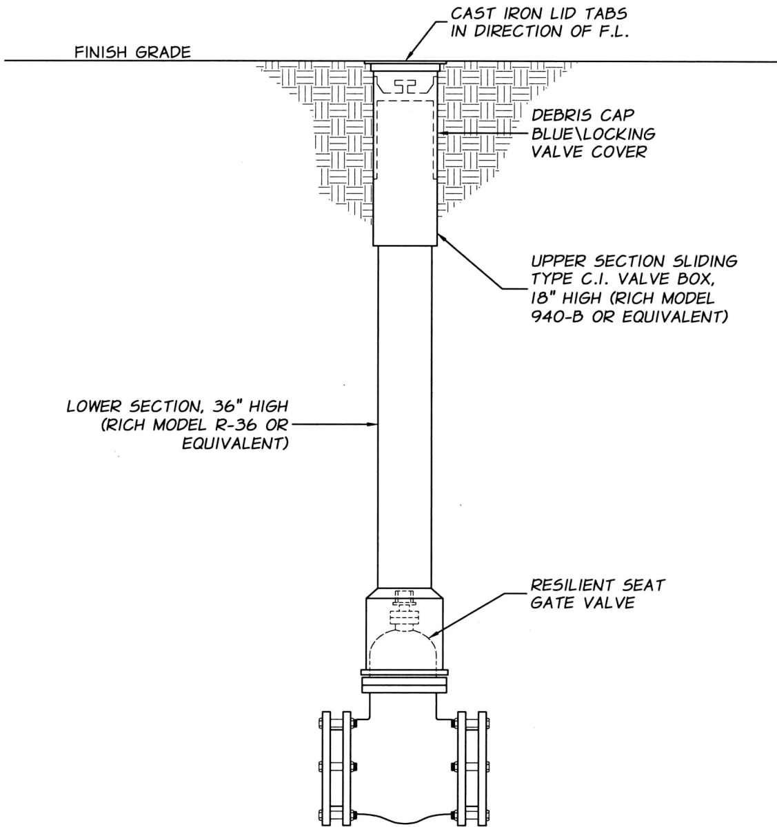
CROSS SECTION NTS
