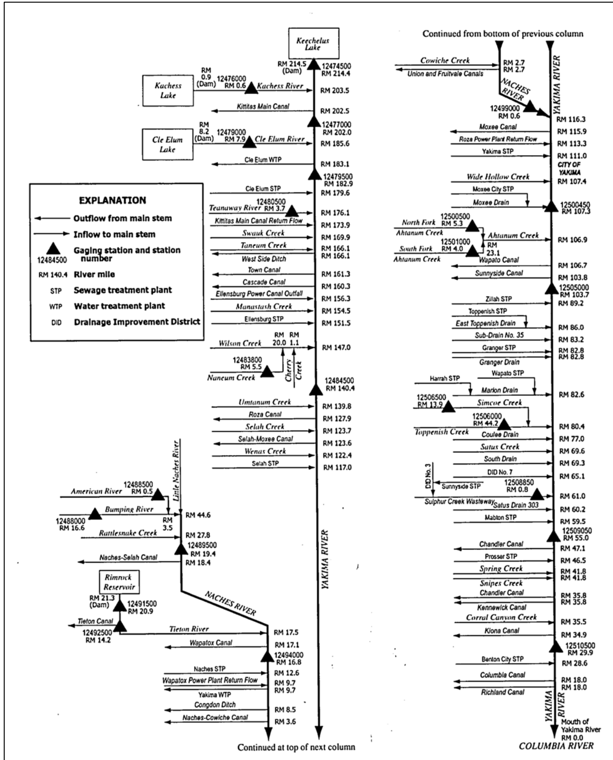
Figure 2-3. Yakima River Basin Schematic. (Source: USGS 1998)
