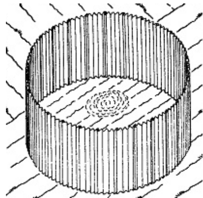
Figure D.9 A ring of steel-sheet piling can alternately be used to ring the boil, if conditions permit.
