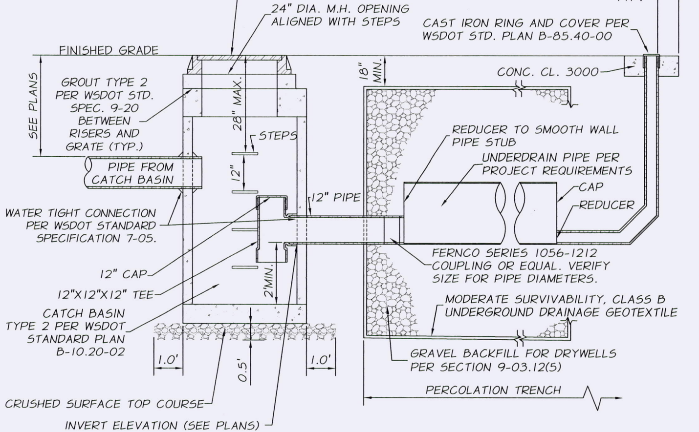
CROSS SECTION NTS
