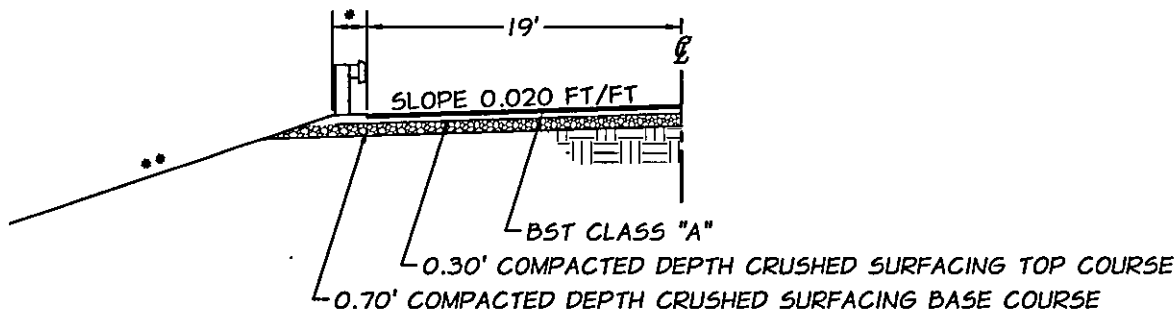
CROSS SECTION NTS
