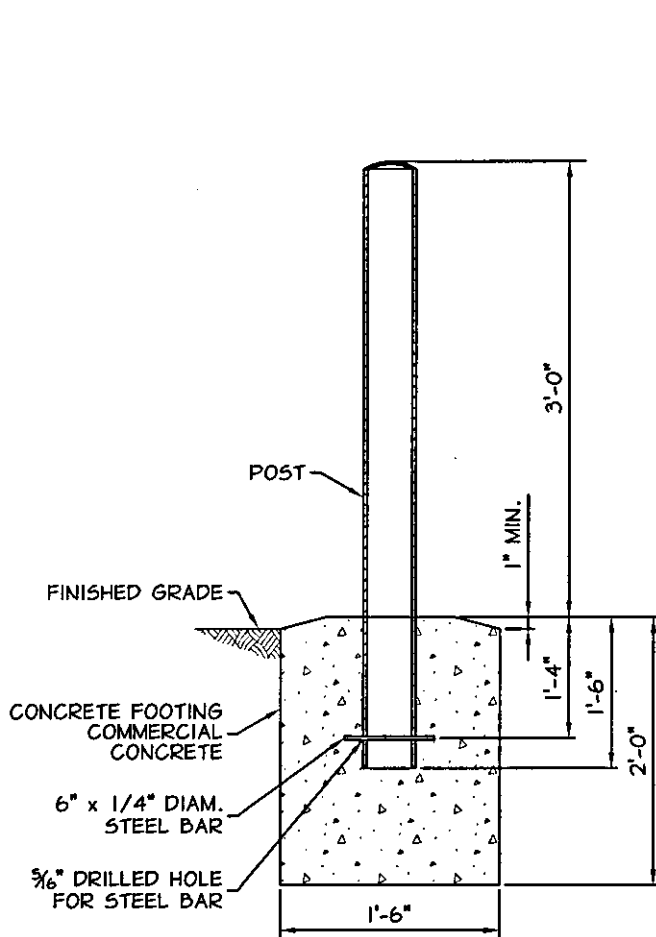
CROSS-SECTION NTS
